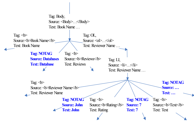
Fig. 8. A WebOQL hypertree for the page p_{e1} in Figure 4.
